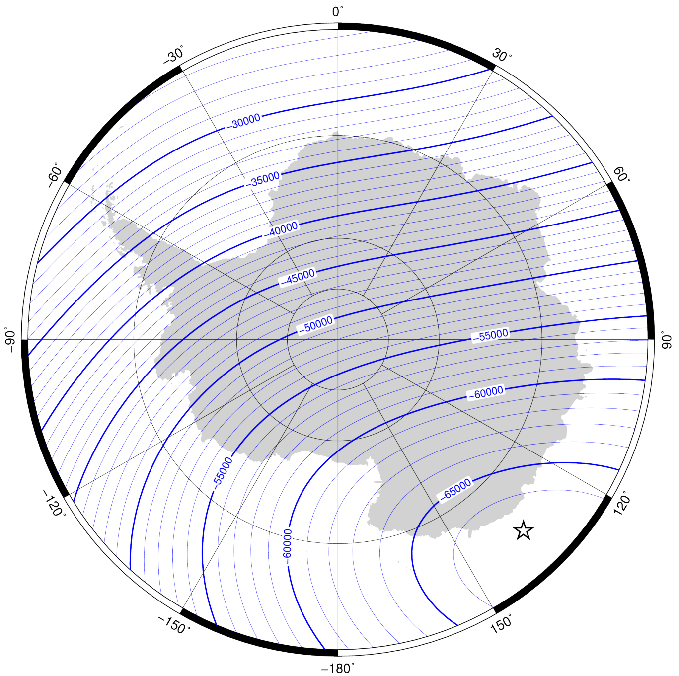
Vertical component ( Z ) in region of south pole at 2020.0 from the World Magnetic Model (WMM2020). Contour interval is 1000 nT, white star is location of a magnetic pole and projection is Polar Stereographic. Credit: British Geological Survey (UK Research and Innovation).
