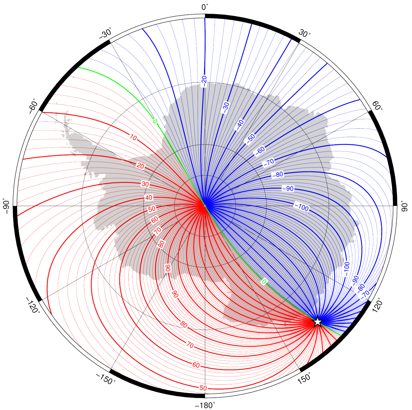
Declination (magnetic variation) in region of south pole at 2020.0 from the World Magnetic Model (WMM2020). Red – positive (east), blue – negative (west), green – zero. Contour interval is 2°, white star is location of a magnetic pole and projection is Polar Stereographic. Credit: British Geological Survey (UK Research and Innovation).
