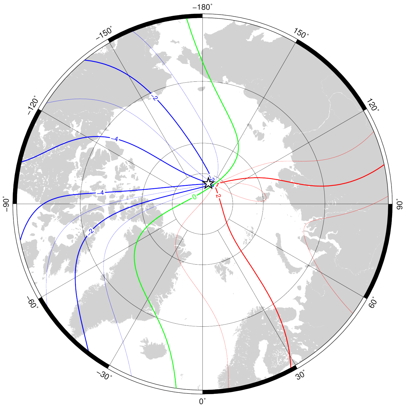
Annual rate of change of inclination in region of north pole for 2020.0 to 2025.0 from the World Magnetic Model (WMM2020). Red – positive change, blue – negative change, green – zero change. Contour interval is 1'/year, white star is location of a magnetic pole and projection is Polar Stereographic. Credit: British Geological Survey (UK Research and Innovation).
