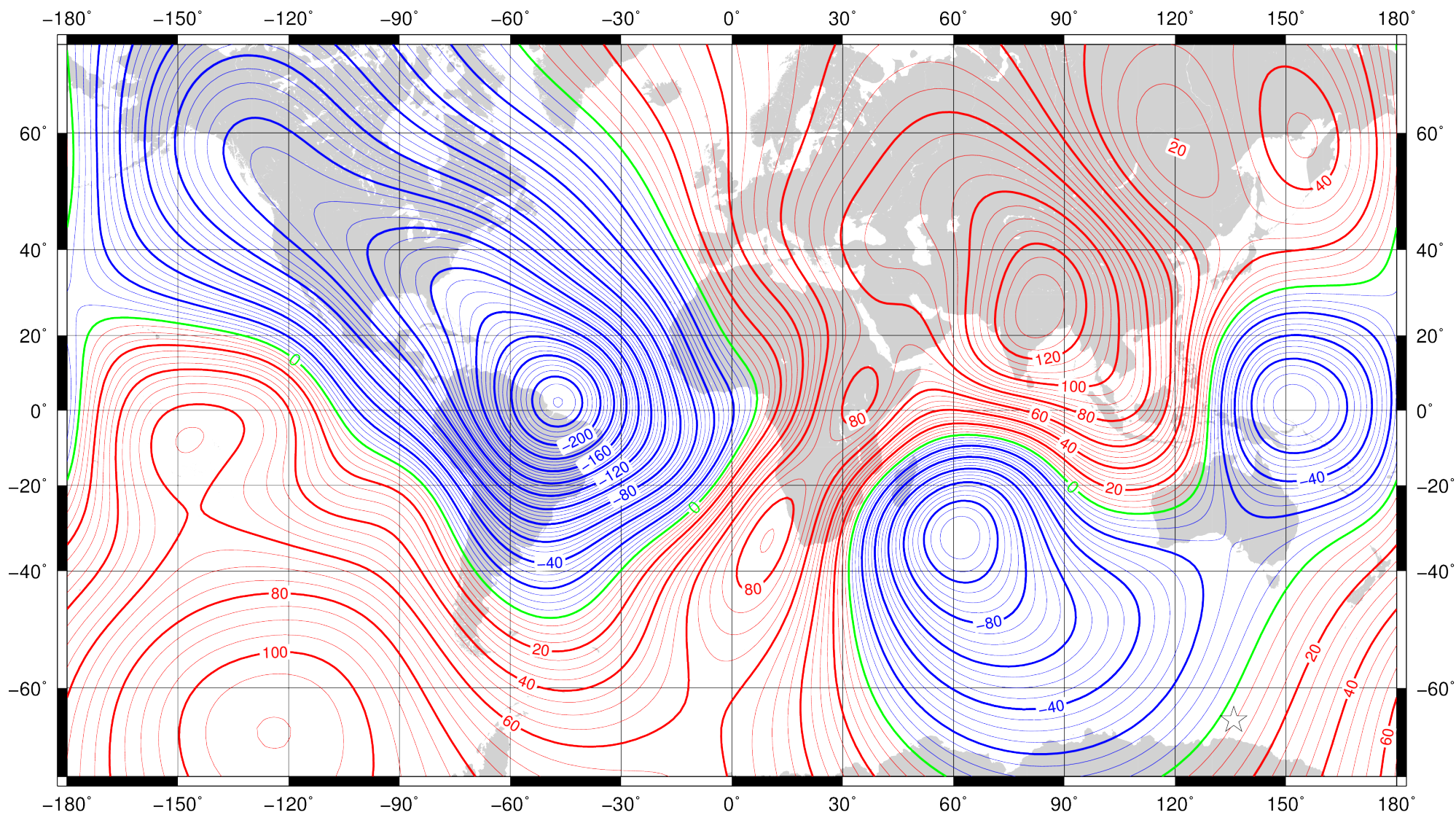
Annual rate of change of vertical intensity for 2020.0 to 2025.0 from the World Magnetic Model (WMM2020). Red – positive change (down), blue – negative change (up), green – zero change. Contour interval is 5 nT/year, white star is location of a magnetic pole and projection is Mercator. This is an example of an isoporic chart. Credit: British Geological Survey (UK Research and Innovation).
