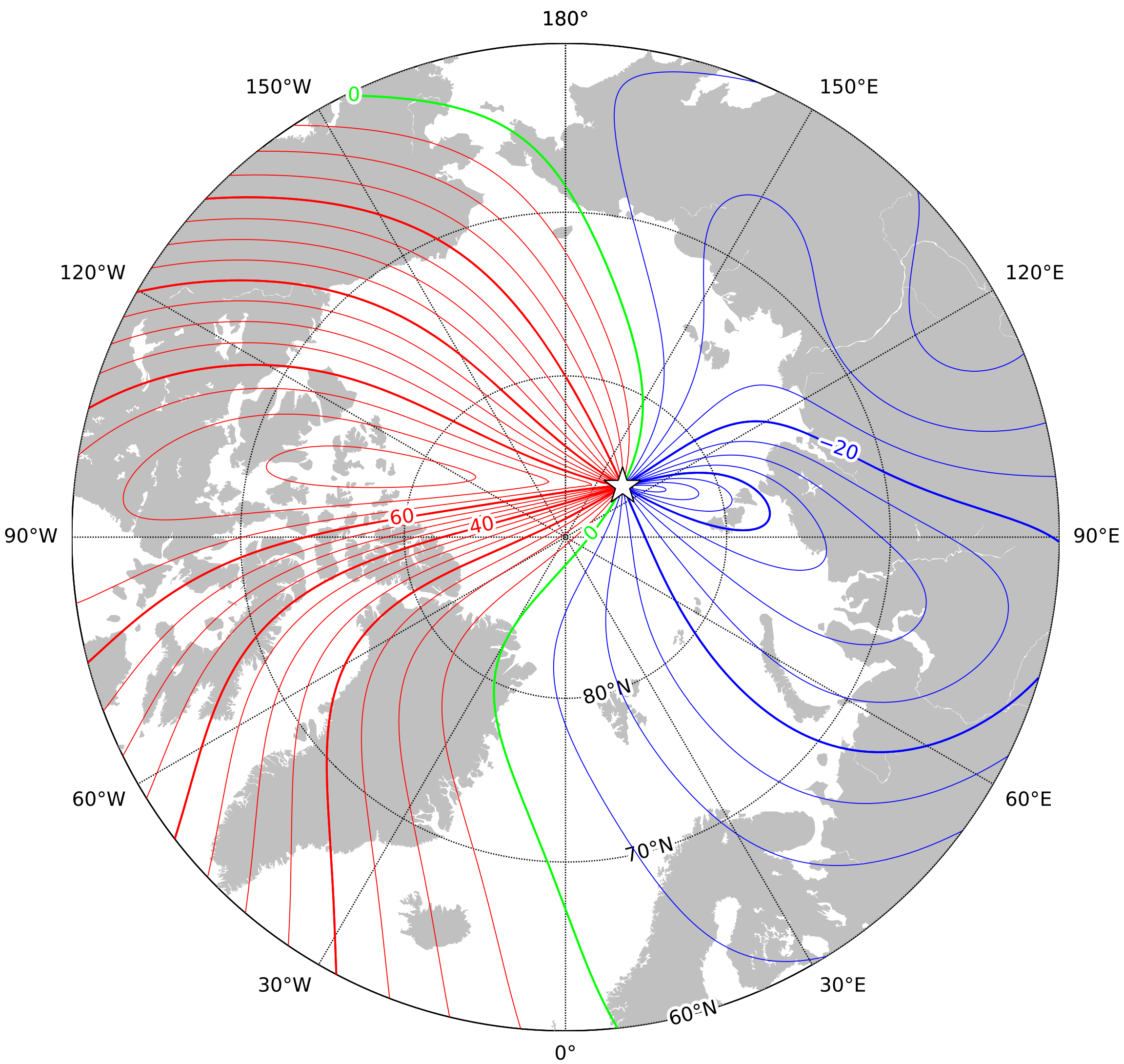
Annual rate of change of horizontal intensity in the region of the north pole at 2027.5 from the World Magnetic Model (WMM) 2025. Red - positive change, blue - negative change, green - zero change. Contour interval is 5nT/year, white star is the location of a magnetic pole and the projection is Polar Stereographic. This is an example of an isoporic chart. British Geological Survey © UKRI 2024
