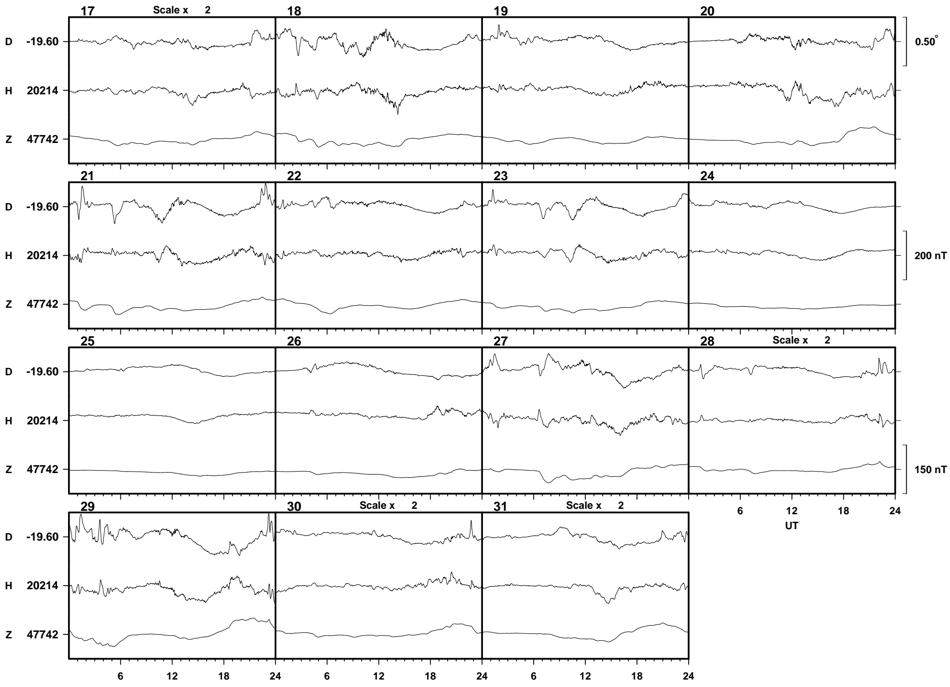
Sable Island March 2003
