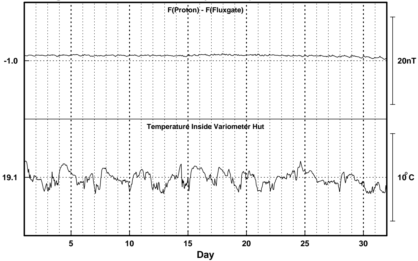
Figure 2 : Sable Island Monthly F Comparison March 2003
