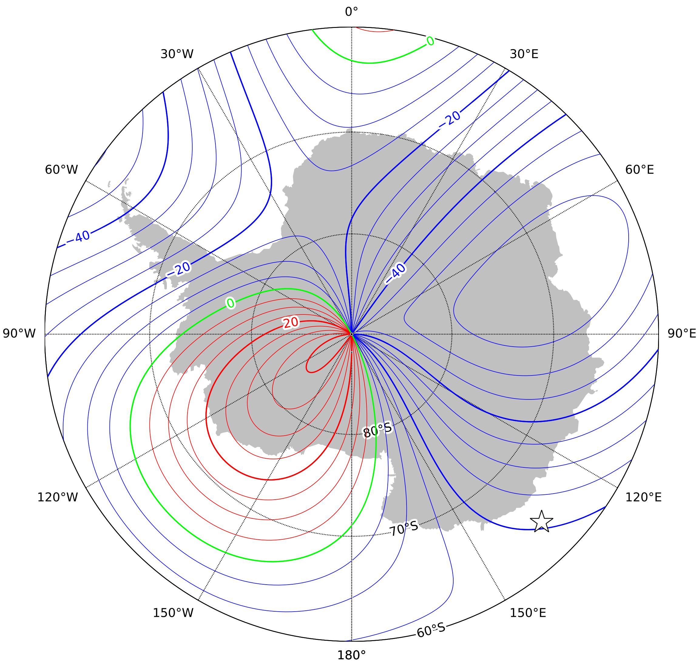
Annual rate of change of north component in the region of the south pole at 2027.5 from the World Magnetic Model (WMM) 2025. Red - positive (northerly) change, blue - negative (southerly) change, green - zero change. Contour interval is 5nT/year, white star is the location of a magnetic pole and the projection is Polar Stereographic. This is an example of an isoporic chart. British Geological Survey © UKRI 2024
