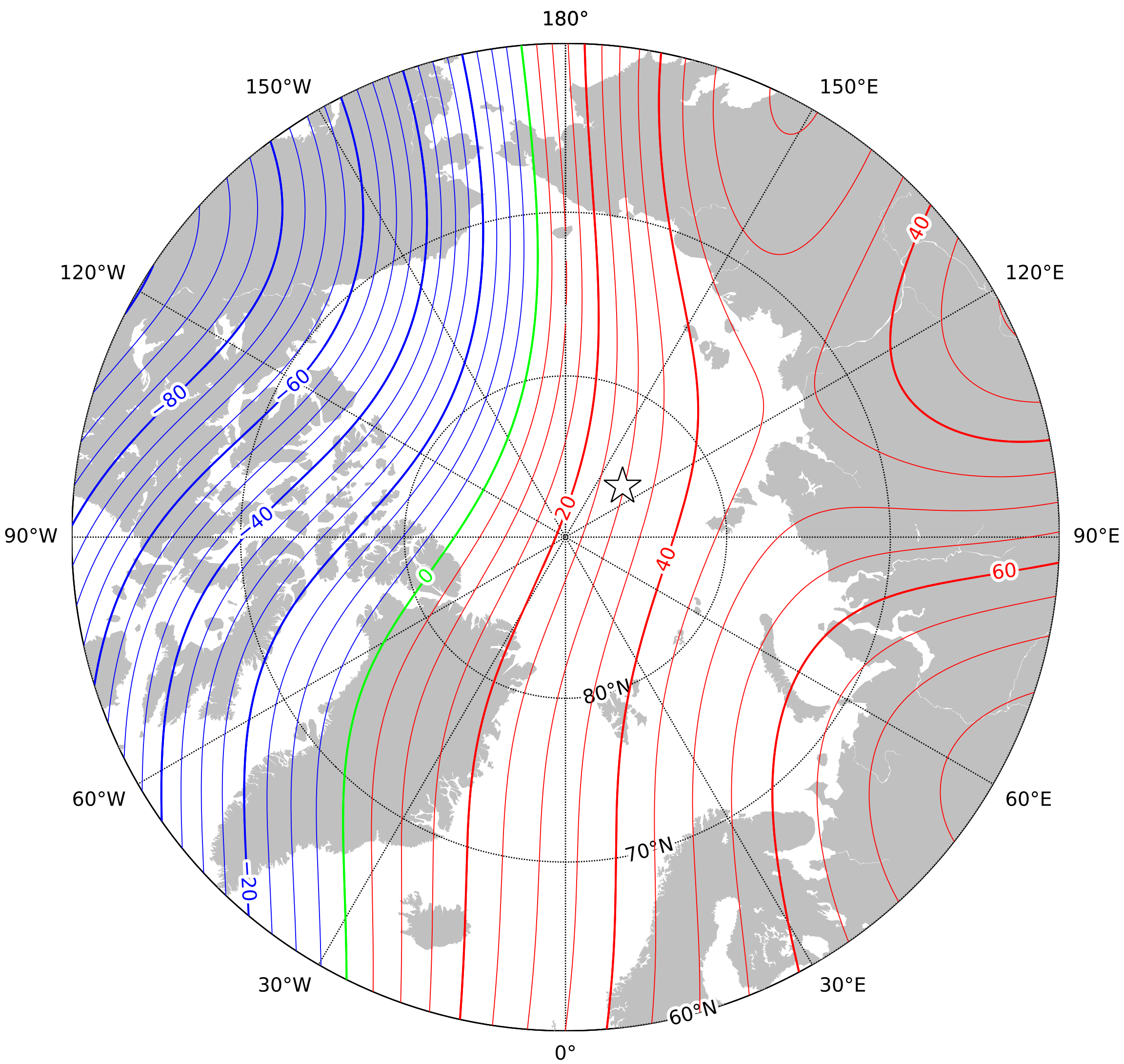
Annual rate of change of downward component in the region of the north pole at 2027.5 from the World Magnetic Model (WMM) 2025. Red - positive (downward) change, blue - negative (upward) change, green - zero change. Contour interval is 5nT/year, white star is the location of a magnetic pole and the projection is Polar Stereographic. This is an example of an isoporic chart. British Geological Survey © UKRI 2024
