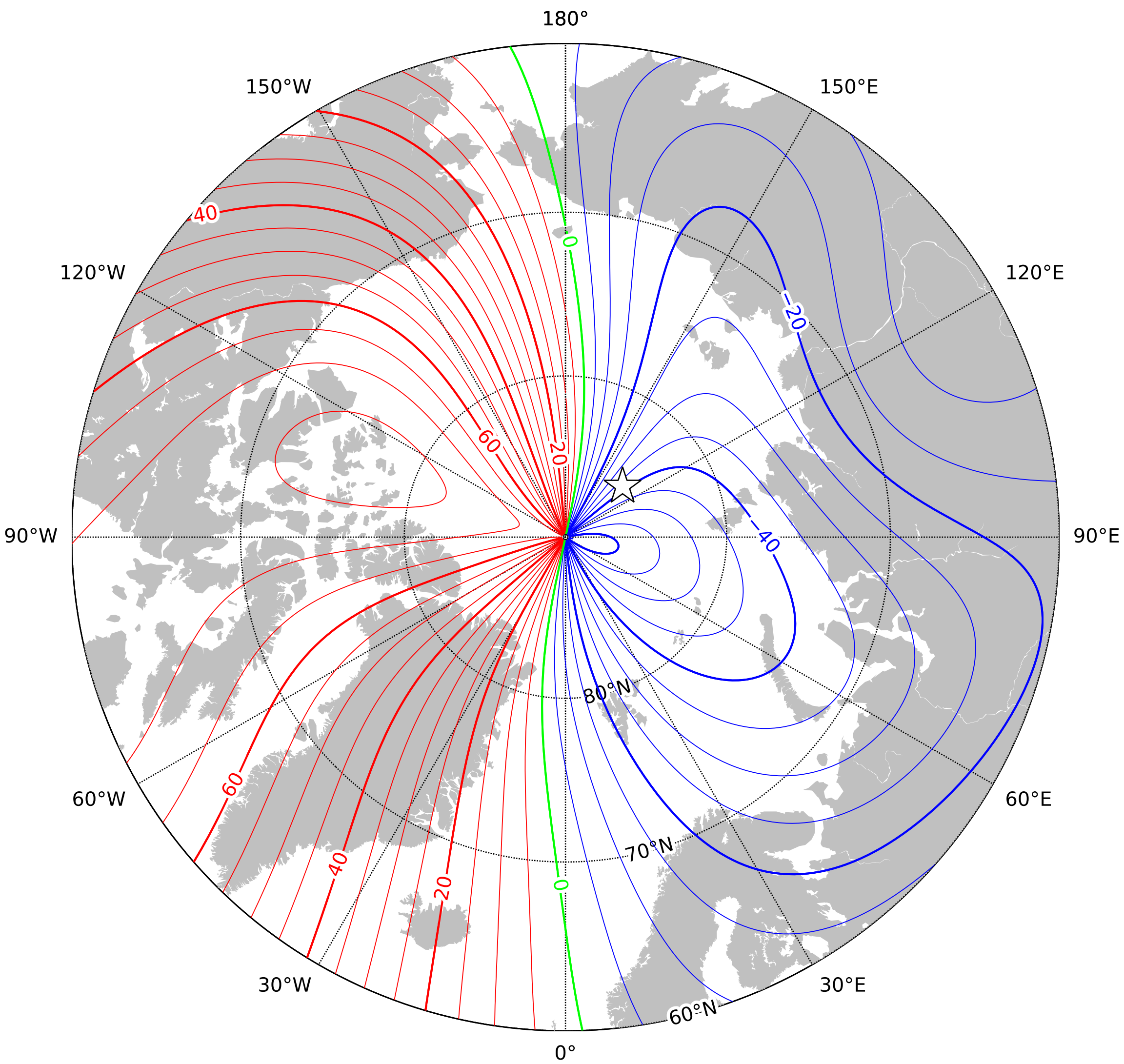
Annual rate of change of north component in the region of the north pole at 2027.5 from the World Magnetic Model (WMM) 2025. Red - positive (northerly) change, blue - negative (southerly) change, green - zero change. Contour interval is 5nT/year, white star is the location of a magnetic pole and the projection is Polar Stereographic. This is an example of an isoporic chart. British Geological Survey © UKRI 2024
