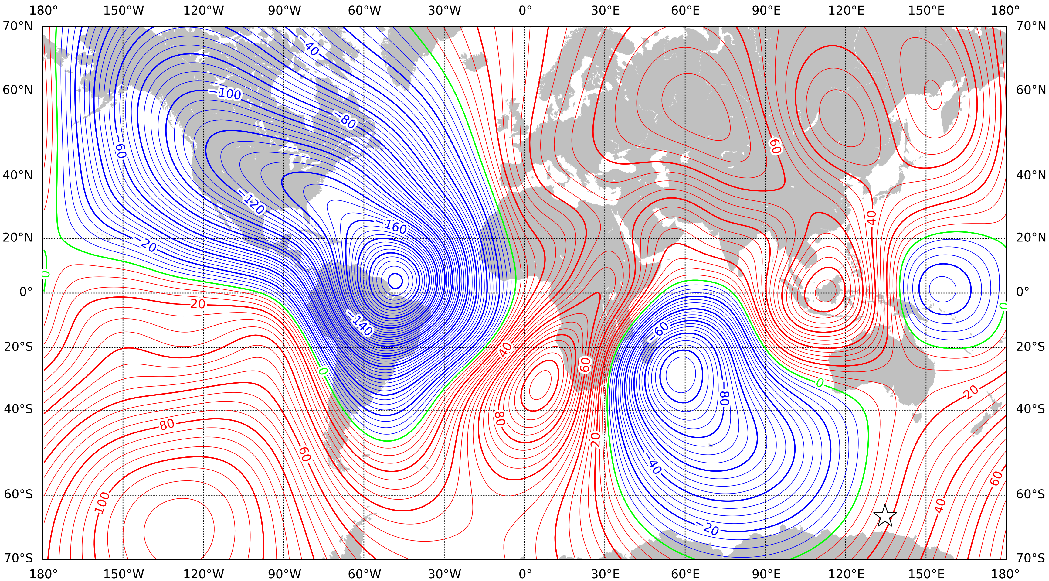
Annual rate of change of downward component at 2027.5 from the World Magnetic Model (WMM) 2025. Red - positive (downward) change, blue - negative (upward) change, green - zero change. Contour interval is 5nT/year, white star is the location of a magnetic pole and the projection is Mercator. This is an example of an isoporic chart.
