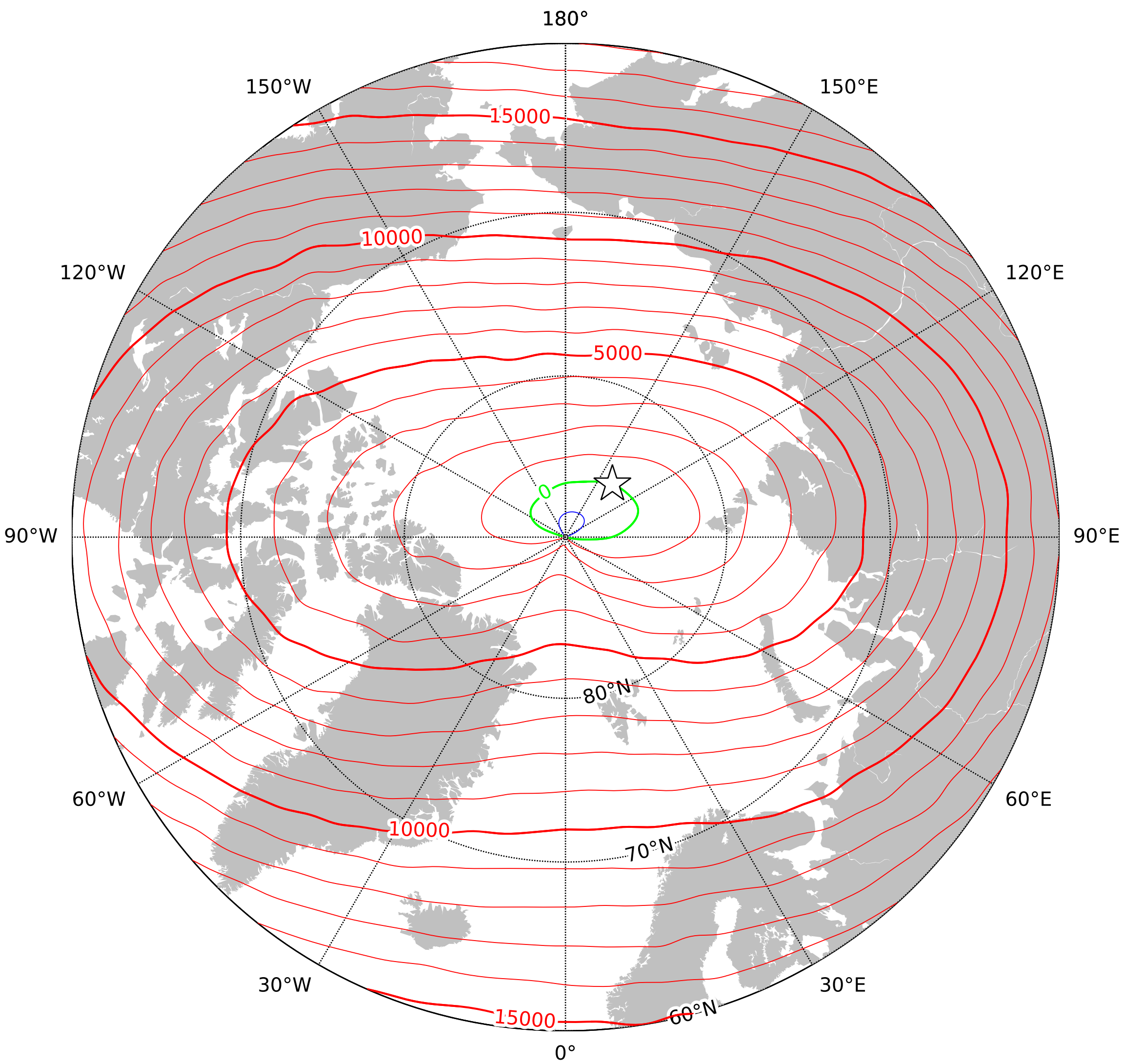
North component (X) in the region of the north pole at 2025.0 from the World Magnetic Model - High Resolution (WMMHR) 2025. Red - positive (north), blue - negative (south), green - zero. Contour interval is 1000nT, white star is the location of a magnetic pole and the projection is Polar Stereographic. This is an example of an isodynamic chart.
